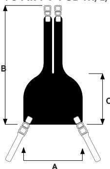
Arnés pélvico en T Tela abeja 3D pelvic harness in 75 AR PV T 3D M/L/XL
